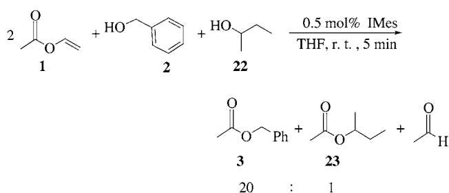
Scheme 3. IMes-Catalyzed Selective Acylation of Benzyl Alcohol
